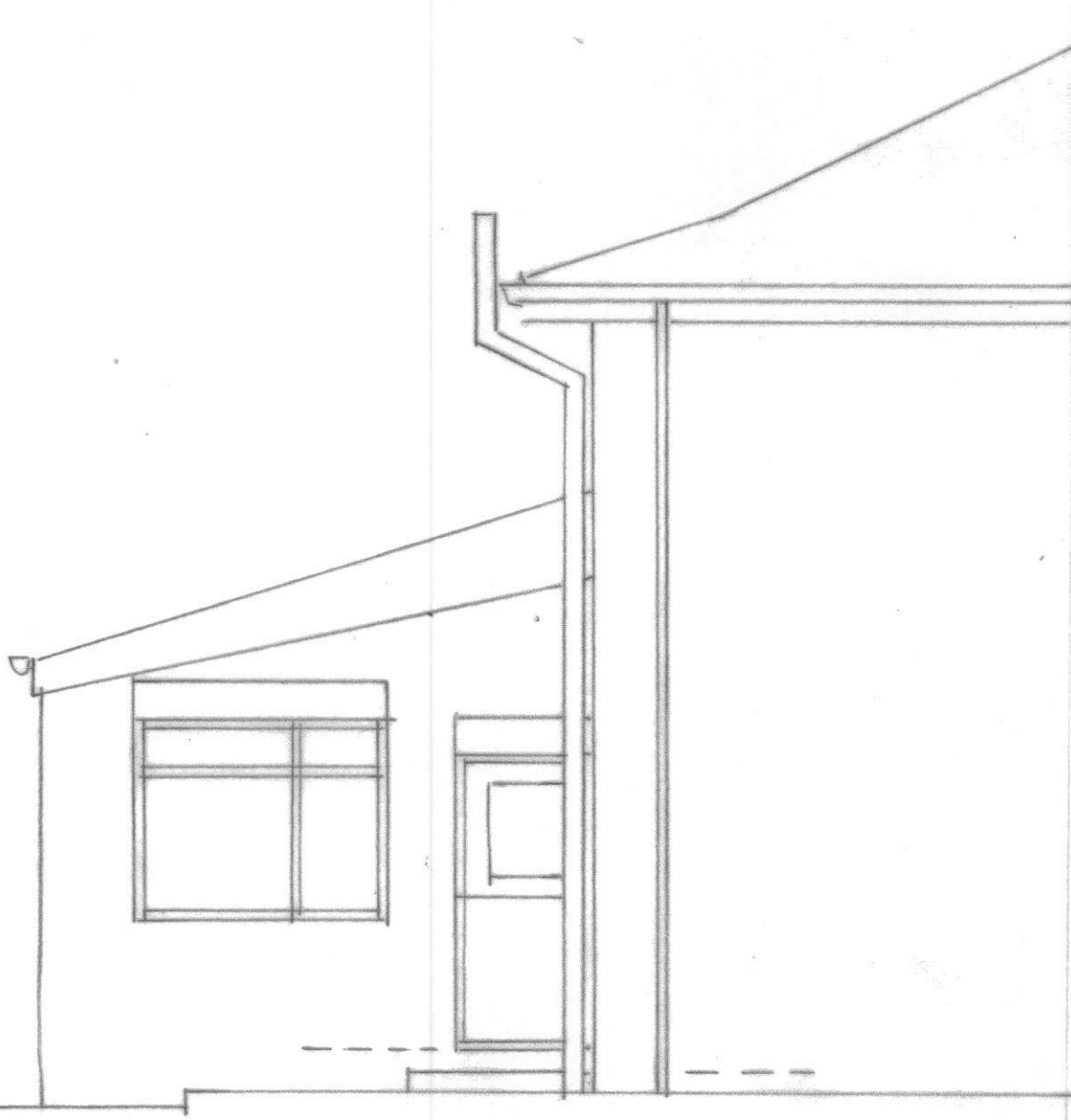
SOUTH ELEVATION
